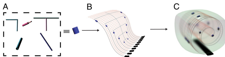
Fig. 1. Strategy for preparing 3D macroporous nanoelectronic networks and integration with host materials. (A) Different nanowire nanoelectronic elements (from left to right): kinked nanowire, nanotube, core-shell, straight, and branched nanowire. (B) Free-standing 2D macroporous nanowire nanoelectronic precursor. Blue, nanoelectronic element; orange, passivation polymer; black, metal contact and input/output. (C) The 3D macroporous nanoelectronic networks integrated with host materials (gray).
