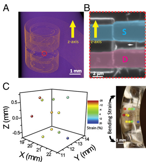
Fig. 5. The 3D macroporous strain sensors embedded in elastomer. (A) Micro-CT 3D reconstruction of the macroporous strain sensor array embedded in a piece of elastomer. Pseudocolors are applied: orange, metal; purple, elastomer. (B) Dark-field microscopy image of a typical nanowire device indicated by red dash circle in A. All of the functional nanowires are intentionally aligned parallel to the axial axis of the elastomer cylinder. The white arrow points to a nanowire. (C) A bending strain field was applied to the elastomer piece. The 3D strain field was mapped by the nanowire strain sensors using the sensitivity calibration of the nanowire devices. The detected strains are labeled in the cylinder image at the device positions.
