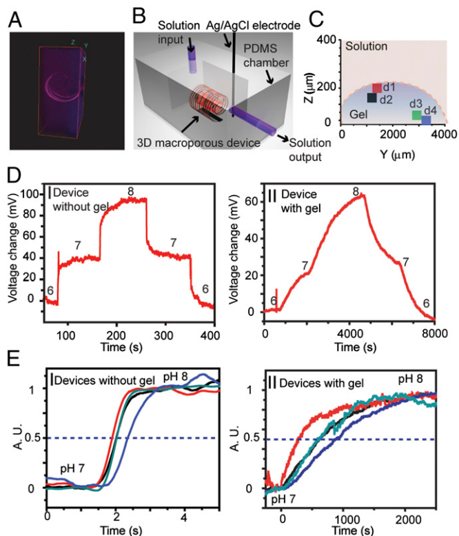
Fig. 4. The 3D macroporous chemical sensors. (A) The xz views of 3D reconstructed image of the 3D macroporous nanoelectronic network in gel. Red (rhodamine 6G), SU-8 mesh network; blue (DAPI), agarose gel. Dimensions: x = 317 \mu\text{m} ; y = 317 \mu\text{m} ; and z = 144 \mu\text{m} . (B) Schematics of the experimental setup. (C) The projection of four nanowire devices in the yz plane. Red dashed line corresponds to the approximate gel boundary, and the red and blue areas correspond to aqueous solution and agarose gel, respectively. (D) Representative change in calibrated voltage over time with pH change for 3D macroporous nanowire chemical sensors (I) in solution and (II) embedded in agarose gel. (E) Calibrated voltage with one pH value change in solution for four different devices located in 3D space. (f) Four devices without gel and (II) four devices embedded in agarose gel.
