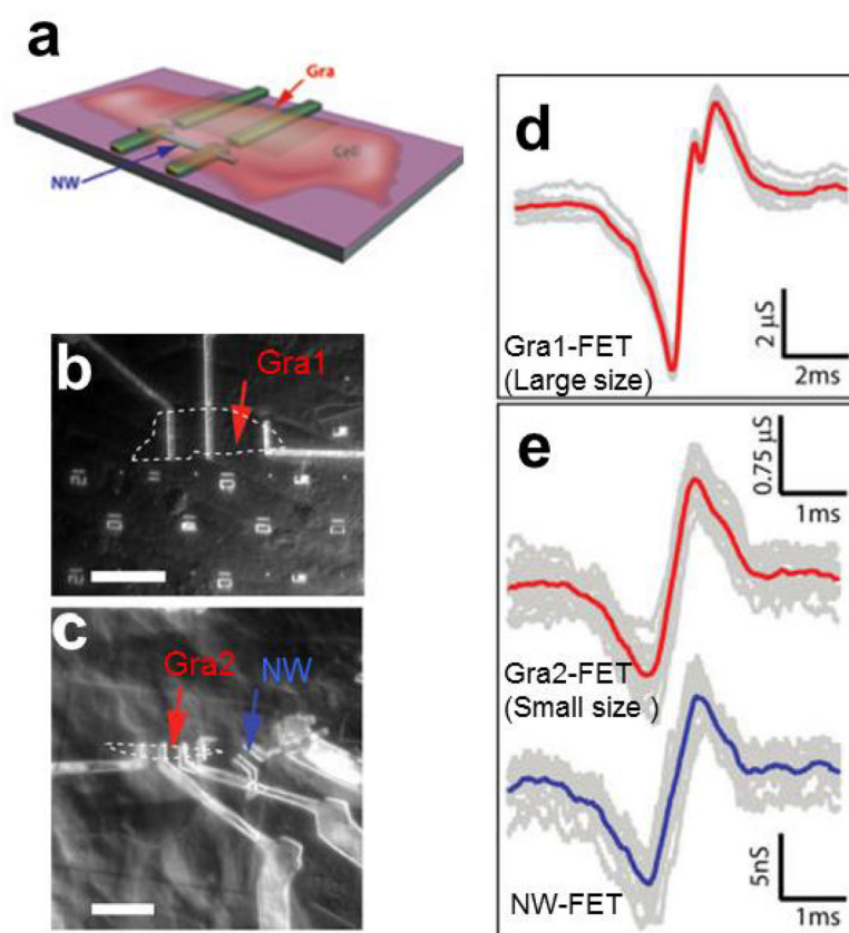
Figure 5. Extracellular action potential recording from nanoFETs with different projection area. (a) Schematic illustrating the chip design incorporating graphene and SiNW FET devices; (b) Optical microscope image of PDMS/cells interfaced with large flake graphene FET. Graphene flake outline is marked by white dashed line; measured device is marked by red arrow. Scale bar is 30 \mu m; (c) Optical microscope image of PDMS/cells interfaced with smaller flake graphene FET and SiNW FET. Graphene flake outline is marked by white dashed line, measured graphene device is marked by red arrow, and measured SiNW device is marked by blue arrow. Scale bar is 13.6 \mu m; (d) Recorded averaged peak (red) and raw data (gray traces) for the Gra1-FET and cell in b ; (e) Thirteen raw signal peaks (gray traces) from the Gra2-FET (upper data) and SiNW FET (lower data) devices marked by red and blue arrows, respectively in c . The average of the peaks was plotted in red and blue, respectively. Reprinted with permission from Ref. [37]. Copyright 2010 American Chemical Society.
